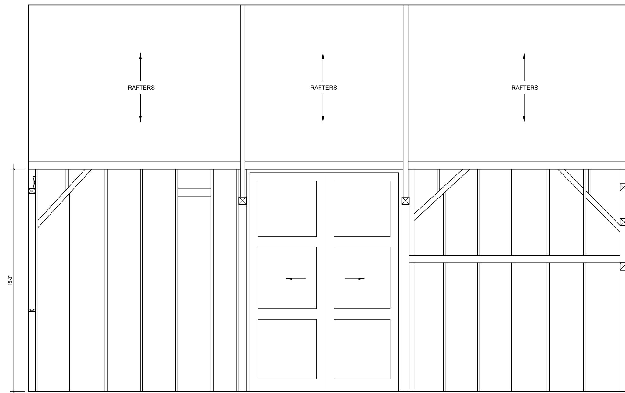
GALLERY Elevation 1 1/4" = 1'-0"
