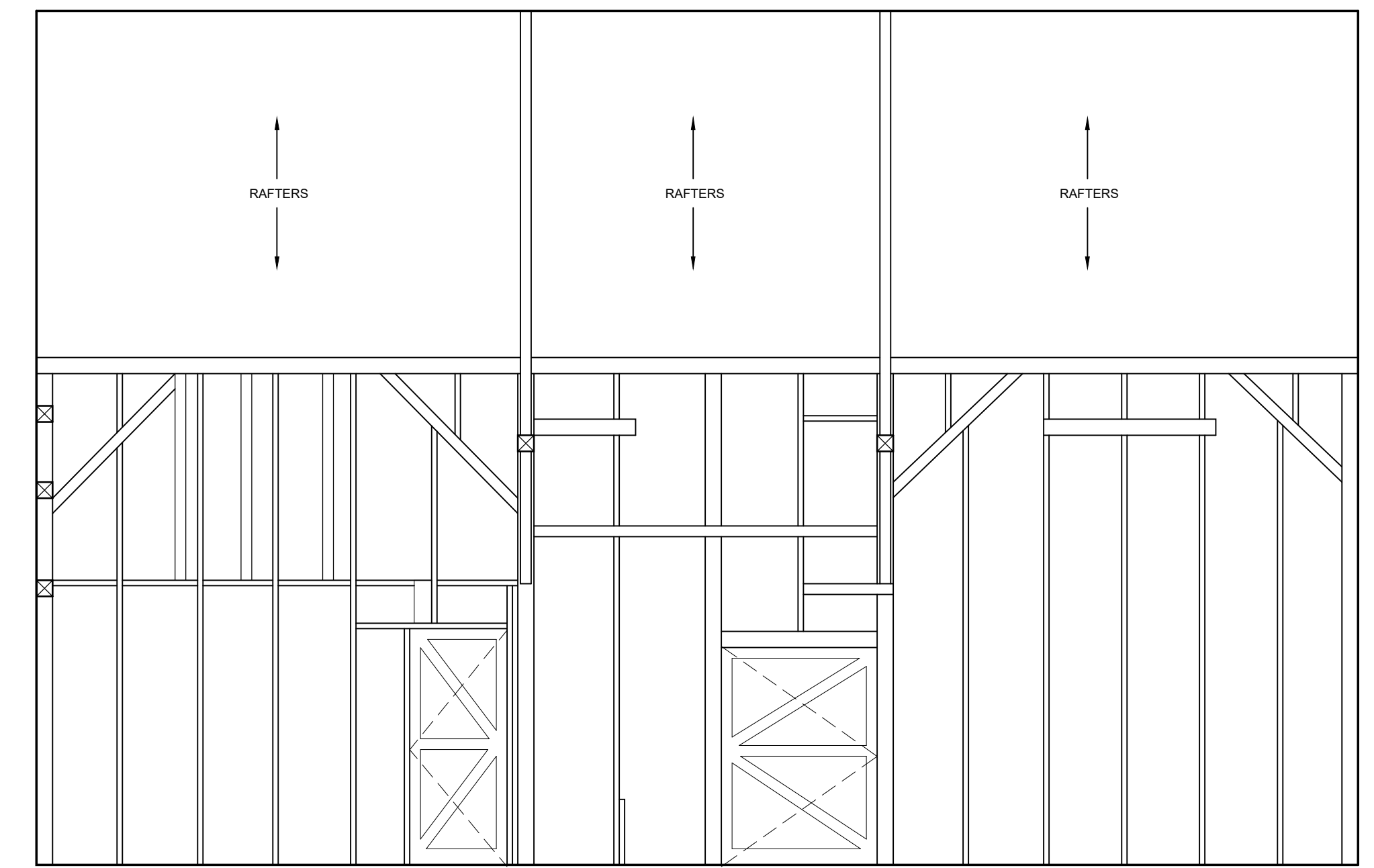
GALLERY Elevation 3 1/4" = 1'-0"
