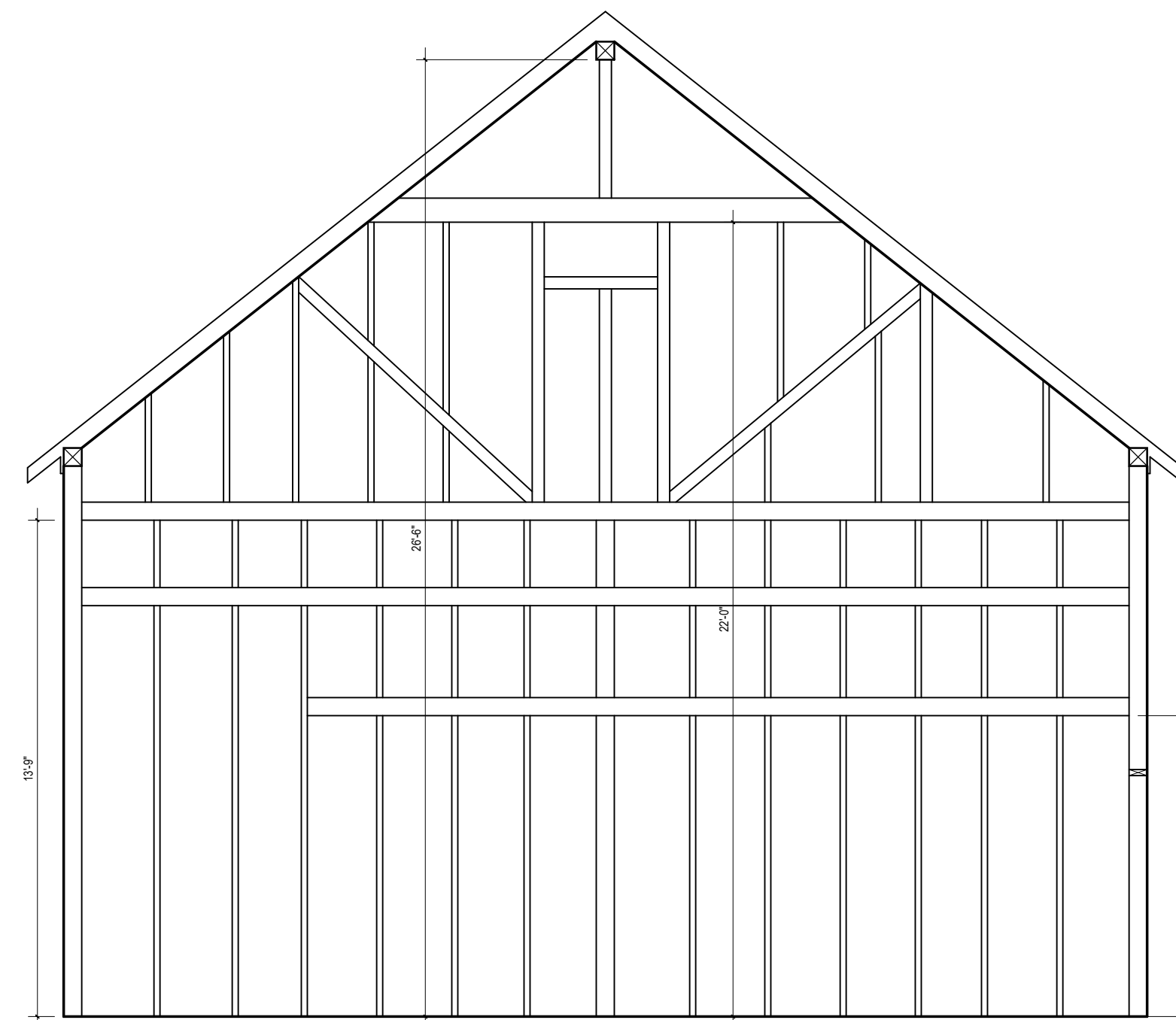
GALLERY Elevation 2 1/4" = 1'-0"
